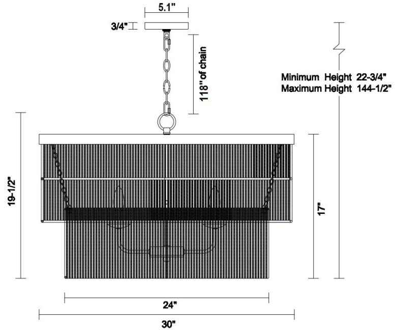
DIMENSION VIEW
