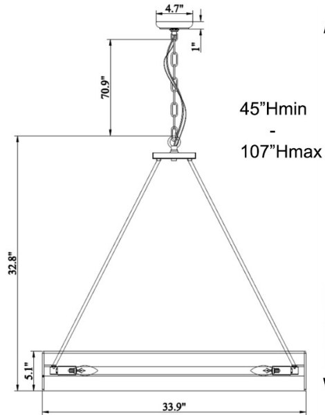
DIMENSION VIEW
