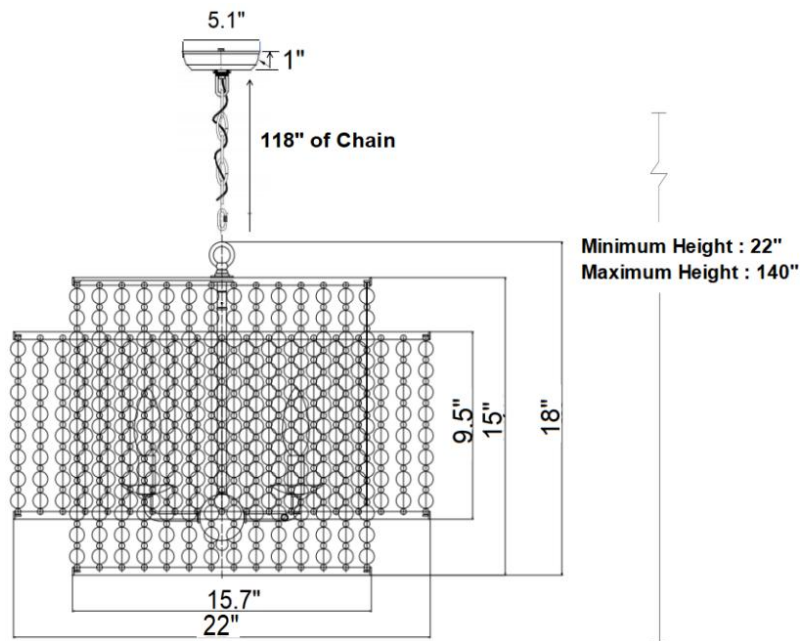
DIMENSION VIEW
