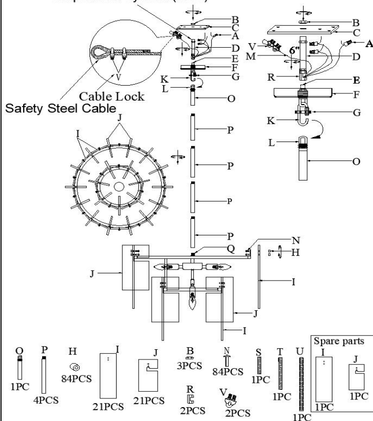
Heavy-Duty Threaded-Pipe Suspension System (HSS)
