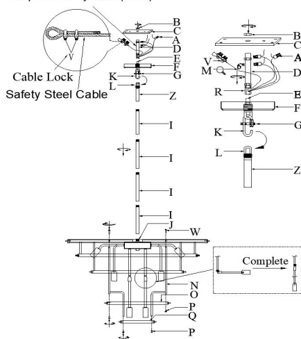
Heavy-Duty Threaded-Pipe Suspension System (HSS)
