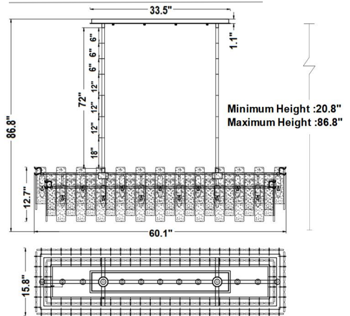
DIMENSION VIEW
