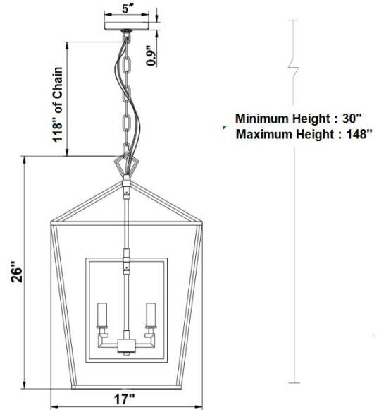
DIMENSION VIEW
