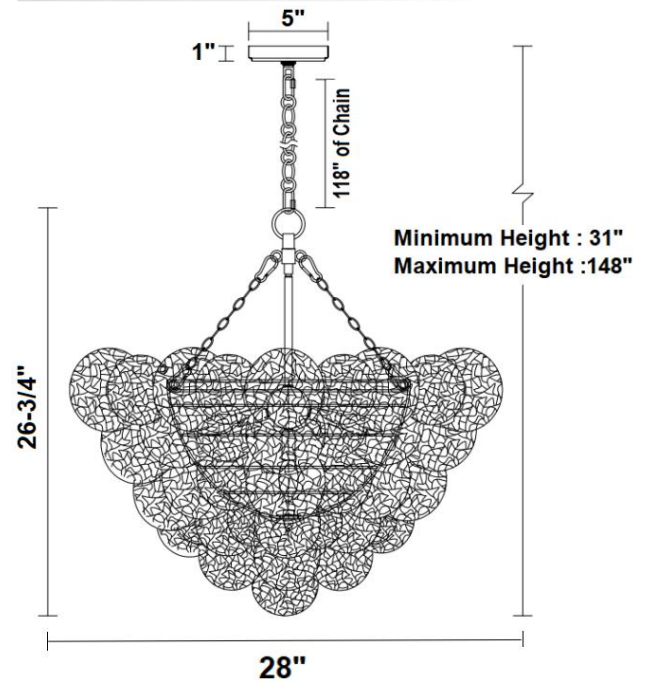
DIMENSION VIEW
