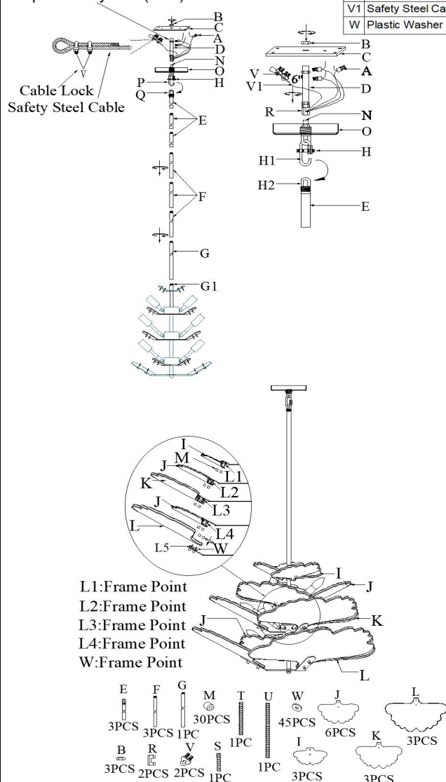
Heavy-Duty Threaded-Pipe Suspension System (HSS)
