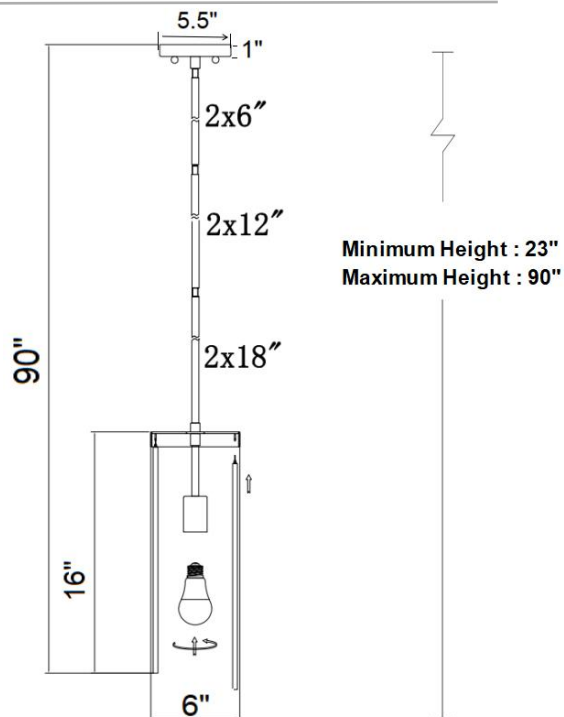
DIMENSION VIEW
