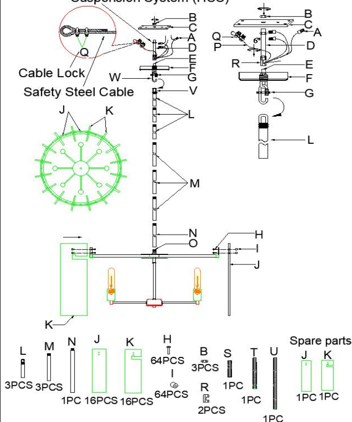
Heavy-Duty Threaded-Pipe Suspension System (HSS)
