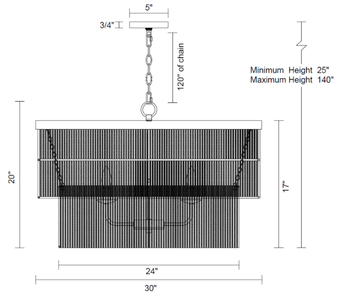
DIMENSION VIEW
