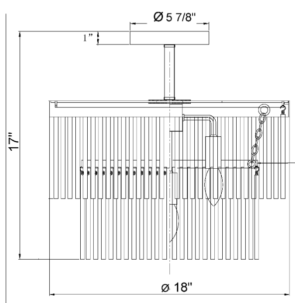
DIMENSION VIEW
