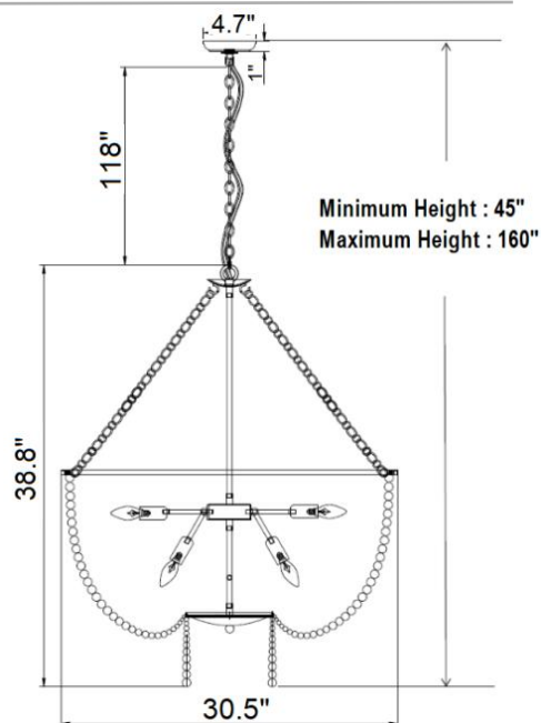
DIMENSION VIEW
